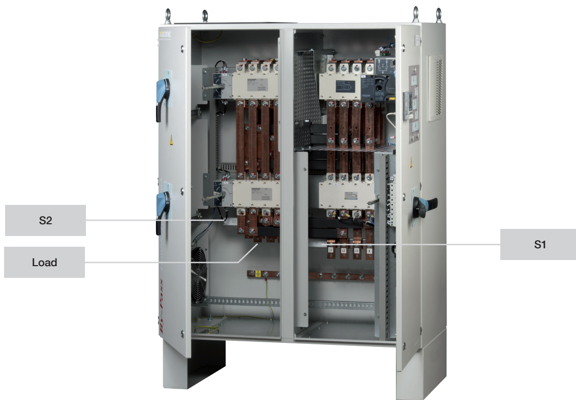
Connection 250 A
