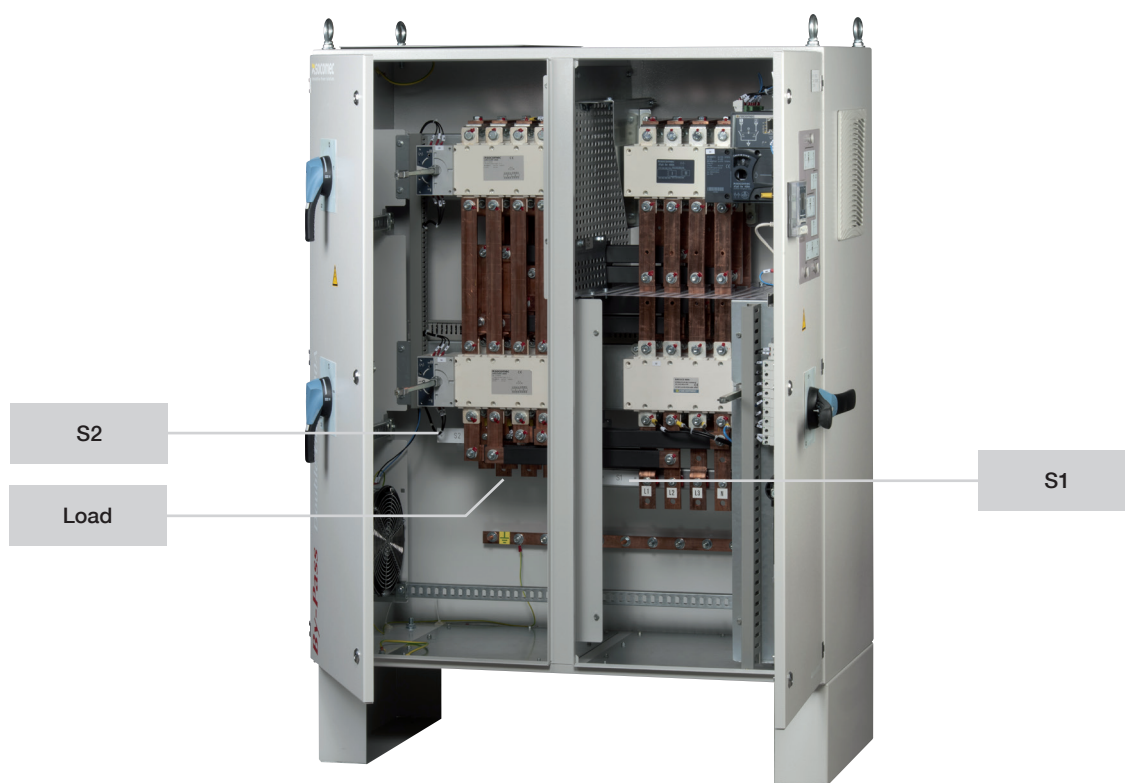
Connection 630 A
