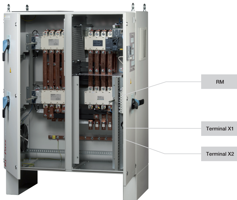
Customer terminal
