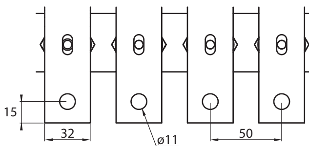
Connection 400 A
