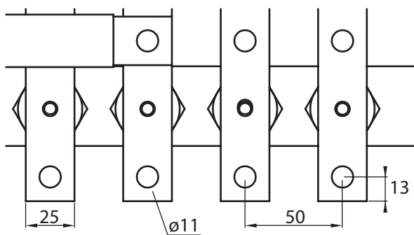
Connection 250 A
