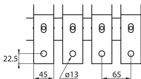
Connection 630 A
